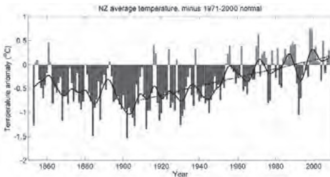
Figure 5. Adjusted average NZ temperatures from 1860 to 2000 as reported by NIWA. ( http://www.niwa.co.nz/our-science/climate/news/all/nz-temp-record )
